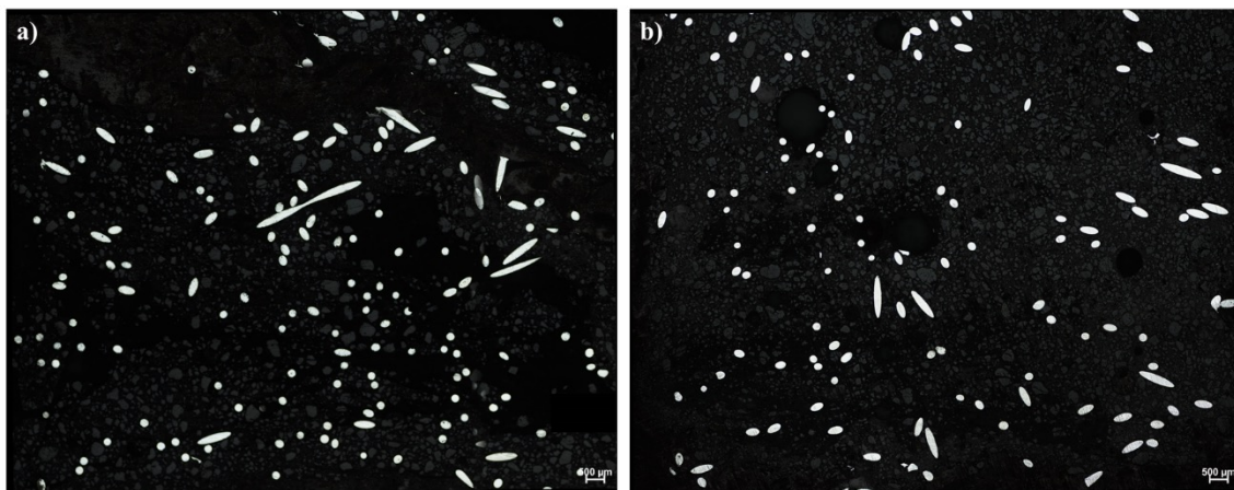
Figure 4. Comparative Image of steel fiber orientation and dispersion of a) F13_226 and b) F13_196.
