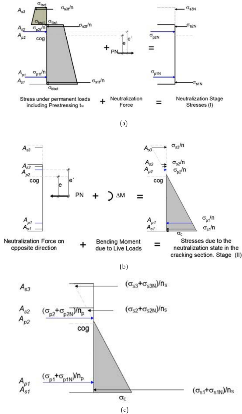
Figure 11: Composite sections at support regions subjected to negative bending in which the top slab is cracked under permanent loads. (a) Stage I: Neutralization of the permanent concrete stresses at the precast beam. (b) Stage II: Increment of stresses from neutralization state due to application of neutralization forces in opposite direction and live loads. (c) Total Stresses: Stages I + II.
