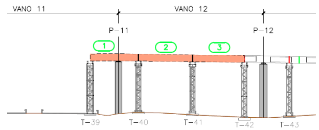
Figure 19. Phase 13: Disassembly of span 12.
