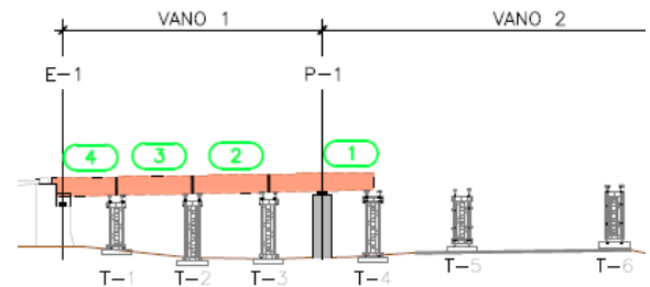
Figure 8. Phase 2: Disassembly of span 1.
