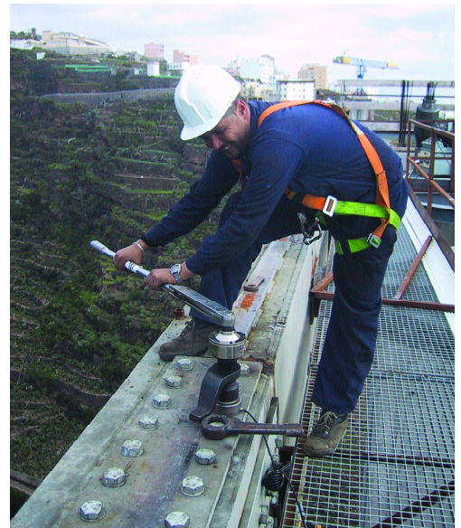
Figura 21. Ensayos preliminares Figure 21. Preliminary tests.
