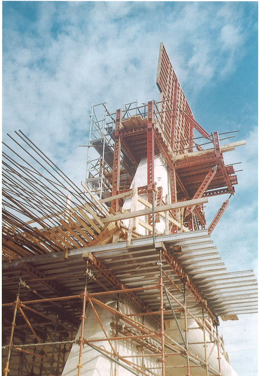
Figura 17. Vano lateral descimbrado Figure 17. Lateral span with falsework already dismantled.
